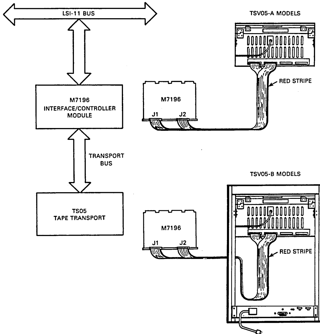
Figure 1-1 TSV05 Subsystem Components
