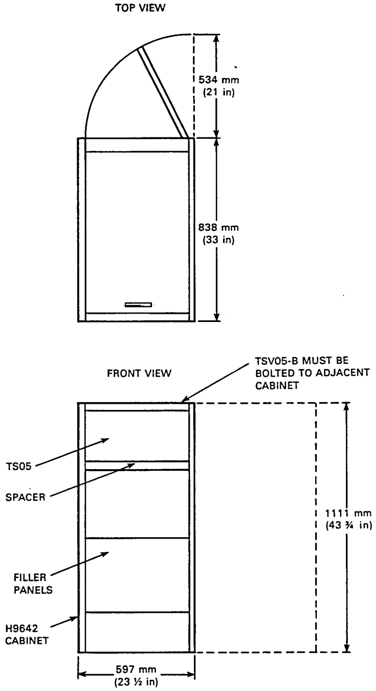
Figure 2-1 Cabinet Access Requirements
