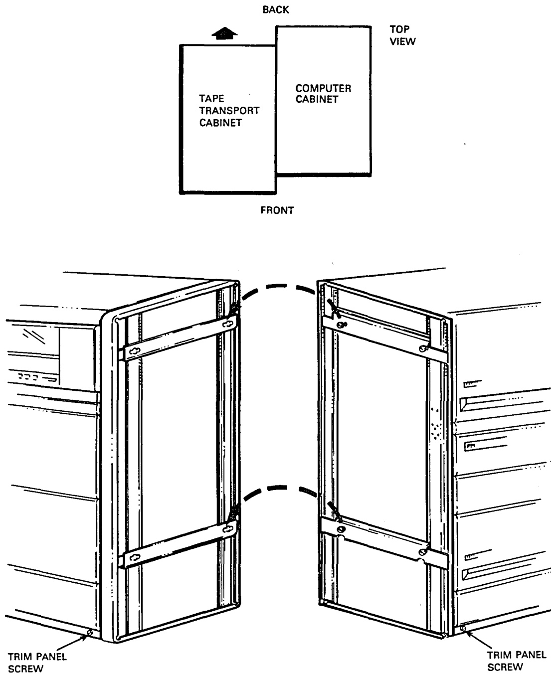
Figure 2-10 Cabinet Alignment
