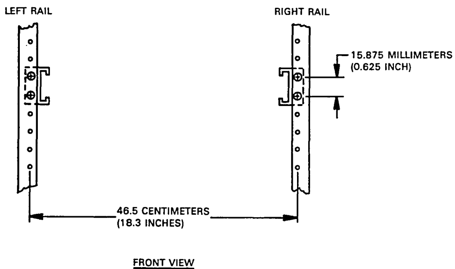
Figure C-2 Chassis Slide Mounting
