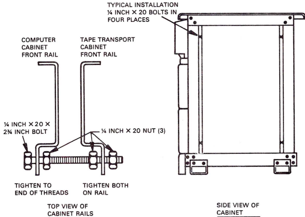
Figure D-1 Cabinet Interconnection
